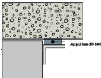
Croquis 2 : Joint solin
