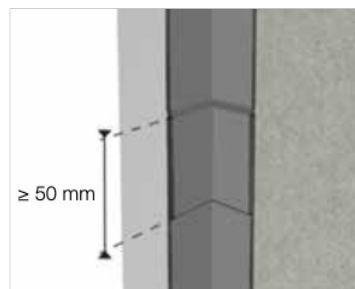
Figure 16 : Raccordement vertical
